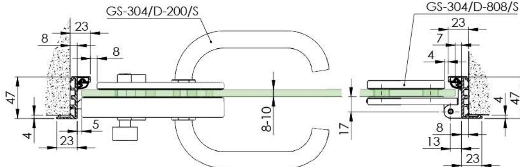
DETAIL B
